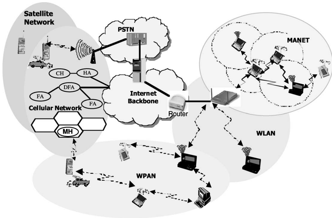
Fig. 1. 4G networks.
