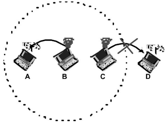
Fig. 5. Exposed-station problem.
