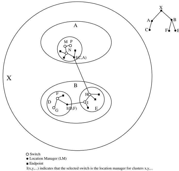
Fig. 1. An example of clustering hierarchy in MMWN.
