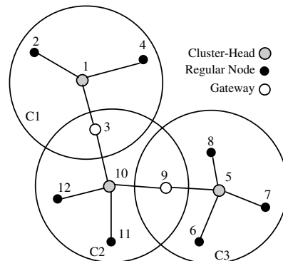
Fig. 2. Illustration of a typical cluster-based network.
