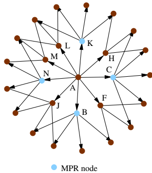
Fig. 4. Multipoint relays.
