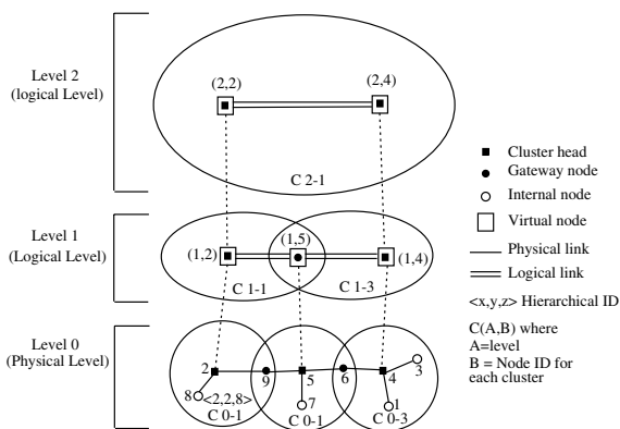
Fig. 3. An example of HSR topology.
